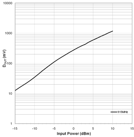
Received Signal Strength Indicator vs. RF_{IN} (dBm)
