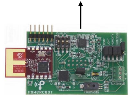
WSN-EVAL-01 Wireless Sensor Board
